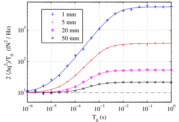
FIG. 2 (color online). Simulation data for the scatter in the total momentum \Delta q transferred to the TM in simulation time T_0 , for several values of the intercylinder gap d , each fit to the model in Eq. (6). The range of gaps studied represents aspect ratios ( 2R/D ) from nearly 7 to 340. The dashed gray line represents the prediction in the limit of infinite gap, S_F^\infty , which is recovered for very short simulation times. Data are scaled for a reference pressure p = 2 \times 10^{-6} Pa.
